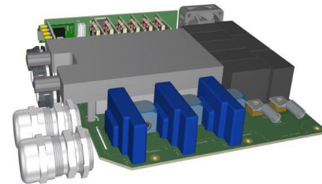
Design of power inverter with hybrid power modules for electric sport car (STU BA)
